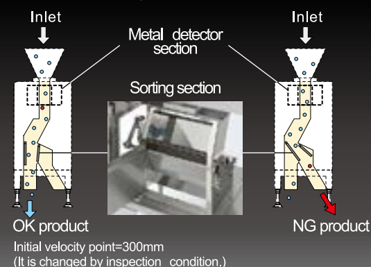
Schematics of sorting operation
